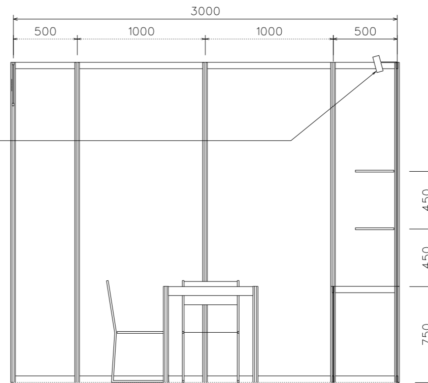
SECTION B
