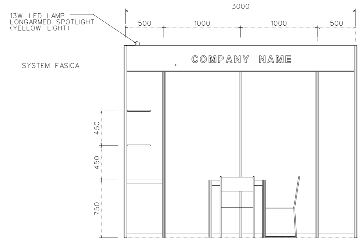
ELEVATION-B
