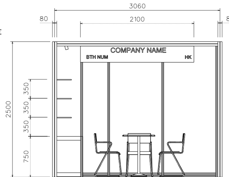
ELEVATION-B
