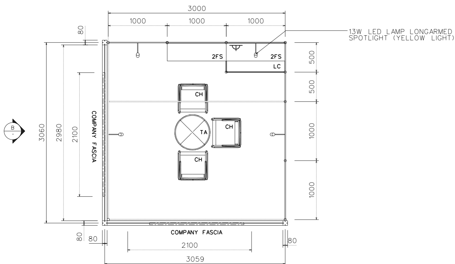
TOP VIEW
