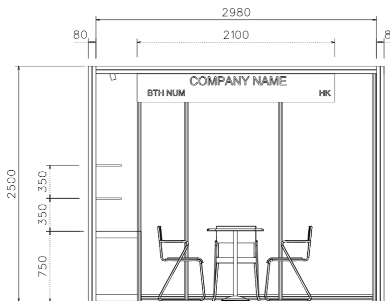
ELEVATION-B
