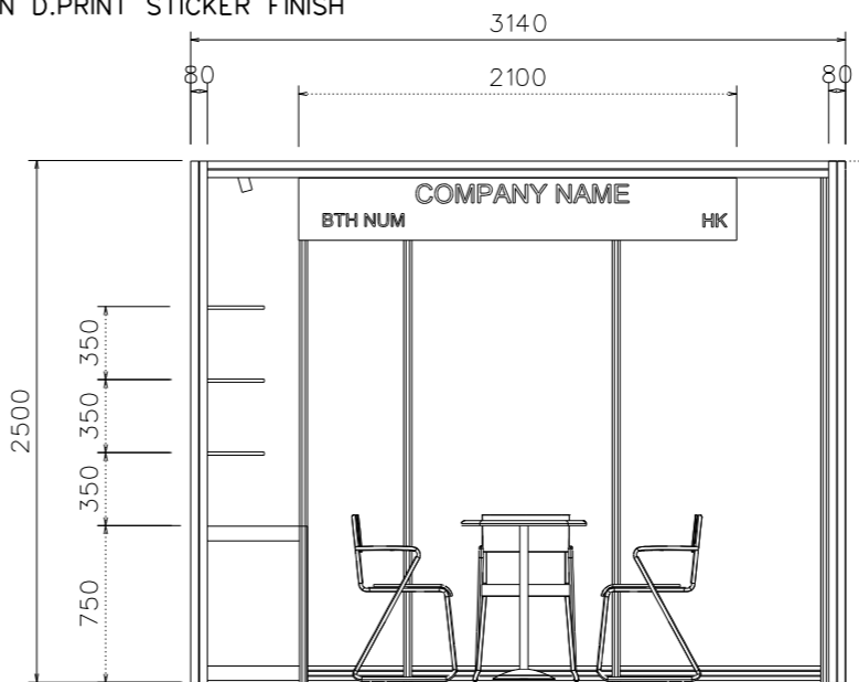
ELEVATION-B
