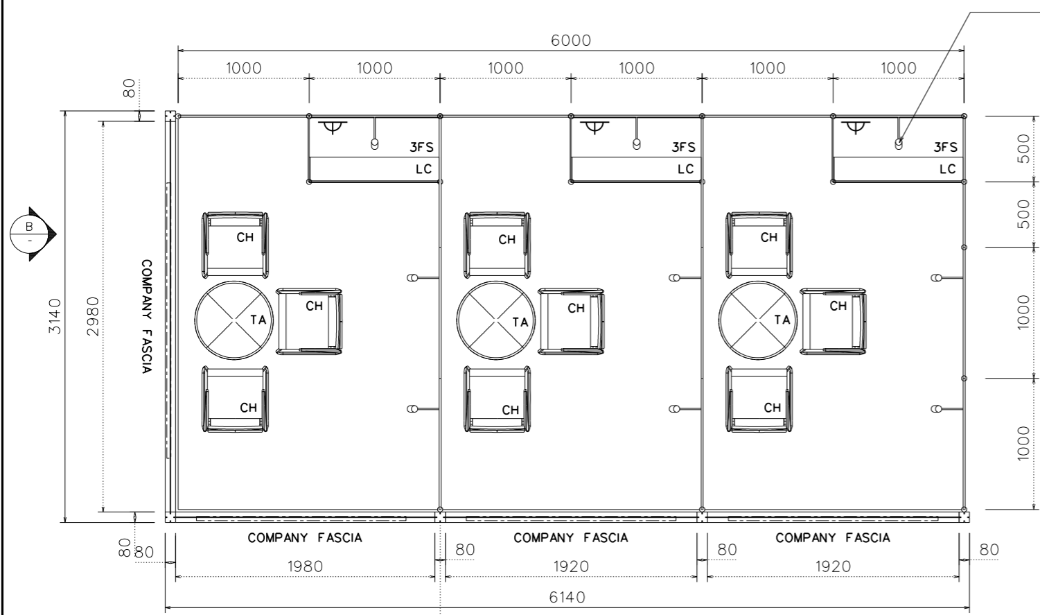
TOP VIEW
