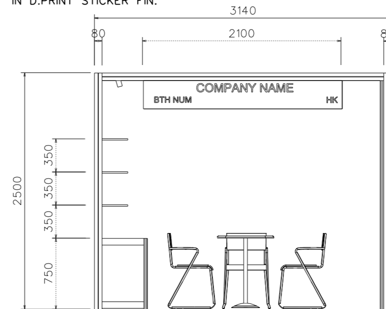
ELEVATION-B
